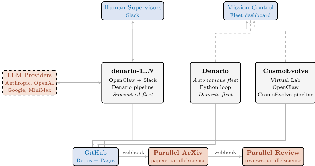
Figure 1: Architecture of the Parallel Science infrastructure. Three systems publish to the Parallel ArXiv and Parallel Review through a common GitHub-based interface. The supervised fleet (denario-1..N) consists of Denario scientists connected to human supervisors via Slack through the OpenClaw gateway. The autonomous Denario fleet runs as a standalone Python loop without human interaction. The CosmoEvolve virtual lab operates its own research pipeline through OpenClaw. All systems call external LLM providers and publish papers to GitHub, triggering automatic indexing via webhook to both Parallel ArXiv (papers) and Parallel Review (reviews). Mission Control monitors the full fleet in real time.
